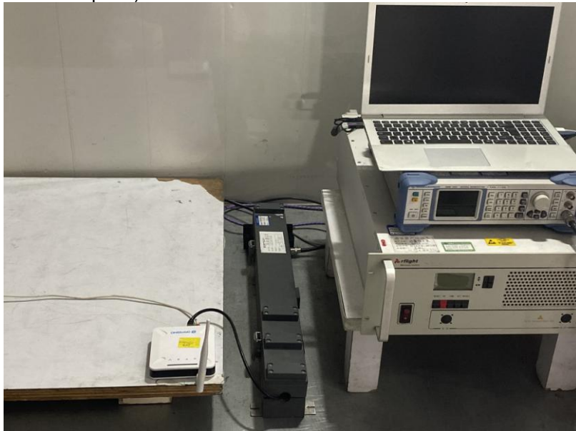
CS(Telecommunication ports)
