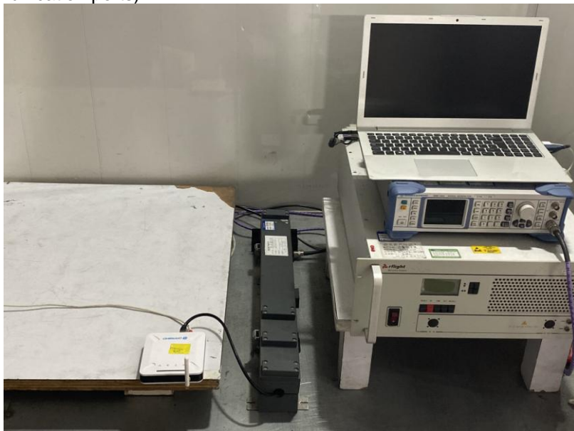
CS(Telecommunication ports)
